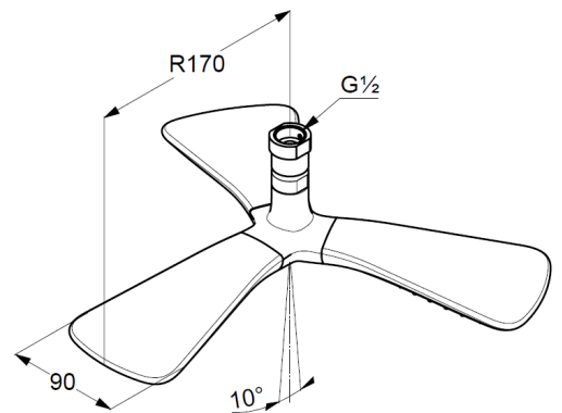
Dimensional drawing
