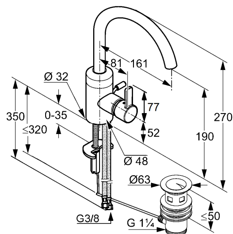
Dimensional drawing
